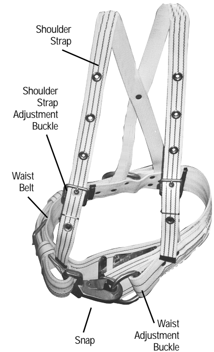
Lewis Snap-on and Cable Reinforced Derrick Belt
